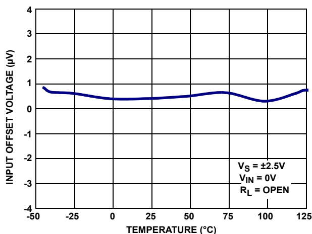
FIGURE 3. V_{0S} vs TEMPERATURE
