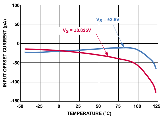
FIGURE 6. I_{0S} vs TEMPERATURE
