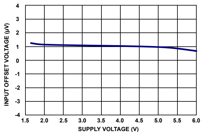
FIGURE 1. V_{0S} vs SUPPLY VOLTAGE
