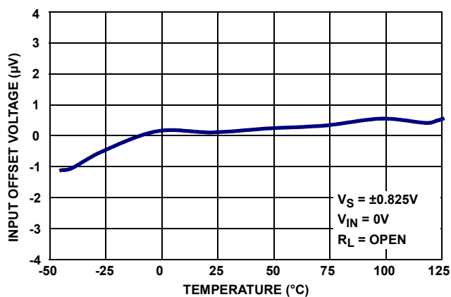
FIGURE 2. V_{0S} vs TEMPERATURE
