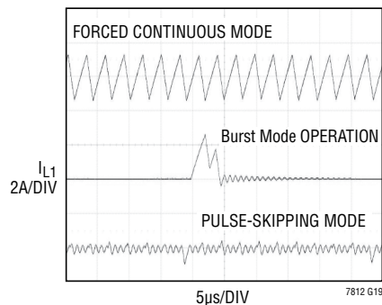
Buck Inductor Current at Light Load
