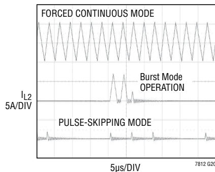
Boost Inductor Current at Light Load
