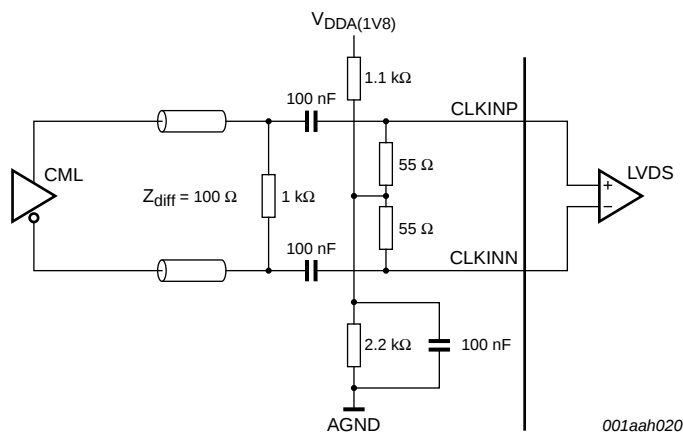
Fig 16. Interfacing CML to LVDS
