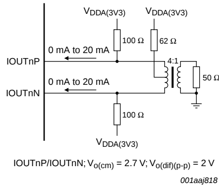
Fig 20. 2 V_{o(p-p)} differential output with transformer
