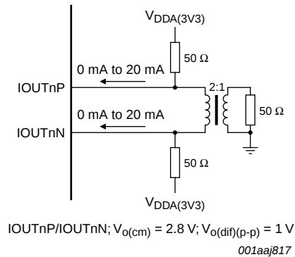
Fig 19. 1 V_{o(p-p)} differential output with transformer
