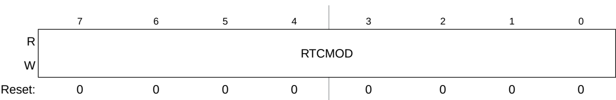
Figure 13-5. RTC Modulo Register (RTCMOD)
