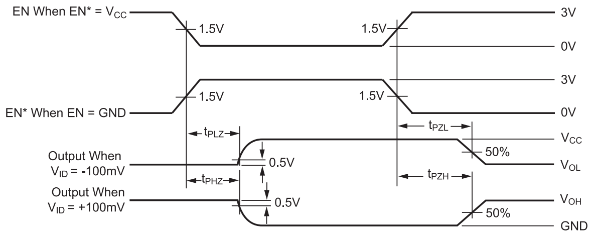
Figure 4. Receiver Three-STATE Delay Waveforms
