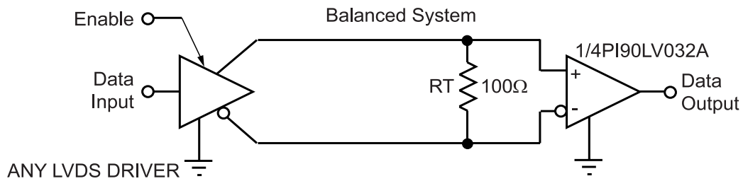
Figure 5. Point-to-Point Application
