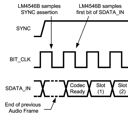
FIGURE 7. Start of AC Link Input Frame
