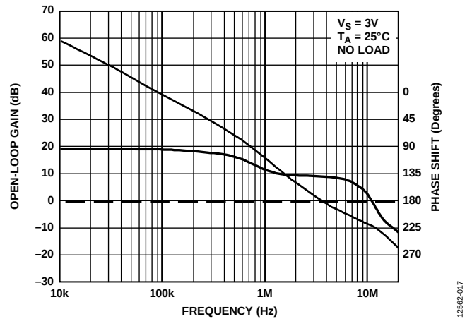
Figure 13. Open-Loop Gain and Phase vs. Frequency (No Load), V_S = 3\text{ V}
