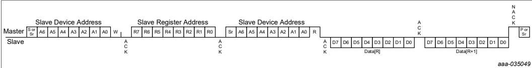
Figure 11. Reading one or more consecutive registers
