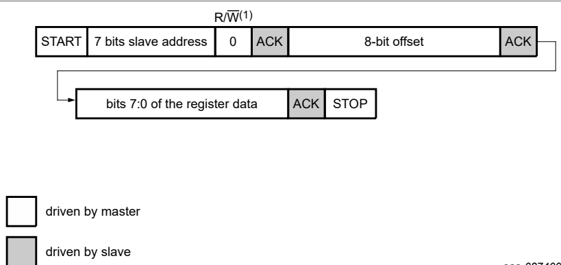
Figure 10. I 2 C write sequence
