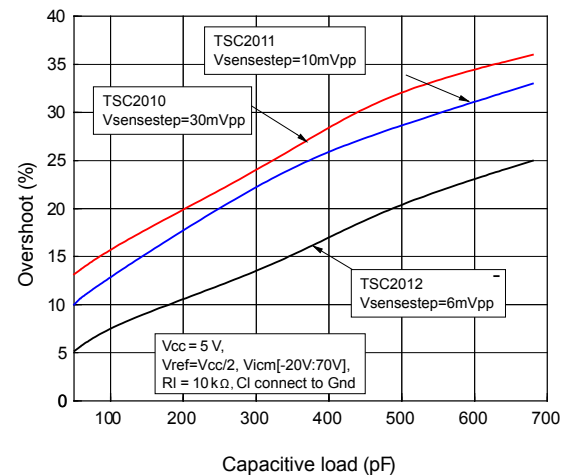
Figure 34. Overshoot vs. capacitive load
