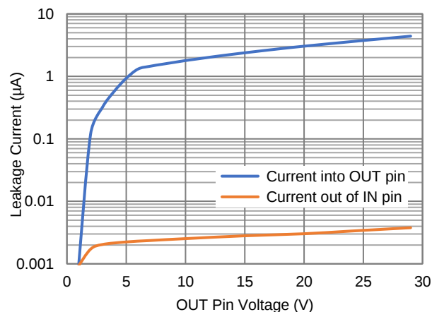
Reverse Leakage Current at OUT Pin (VIN = GND, \overline{EN} = \text{high} )
