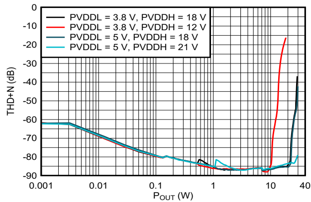
Figure 6-4. THD+N vs Output Power
