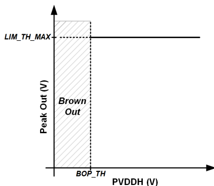
Figure 8-1. Limiter with Fixed Threshold
