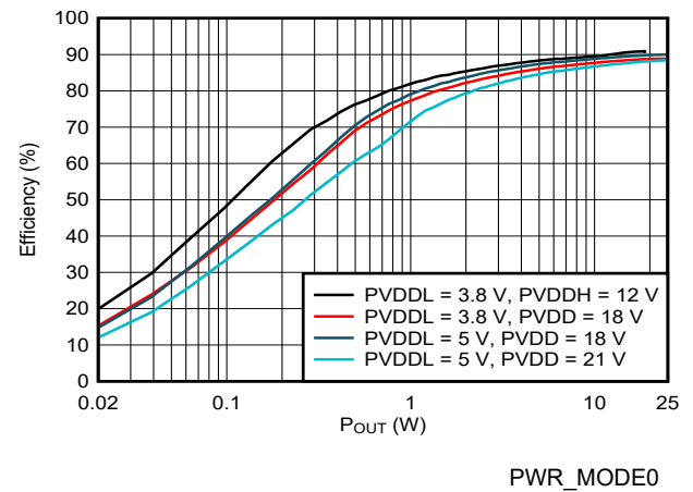
Figure 9-6. Efficiency vs Output Power
