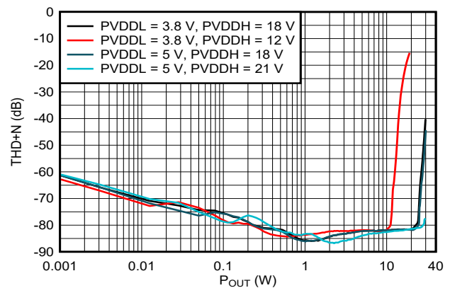
Figure 6-5. THD+N vs Output Power
