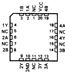
SN54F36 . . . FK PACKAGE (TOP VIEW)
