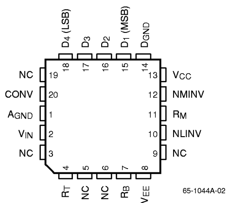
20 Lead PLCC
