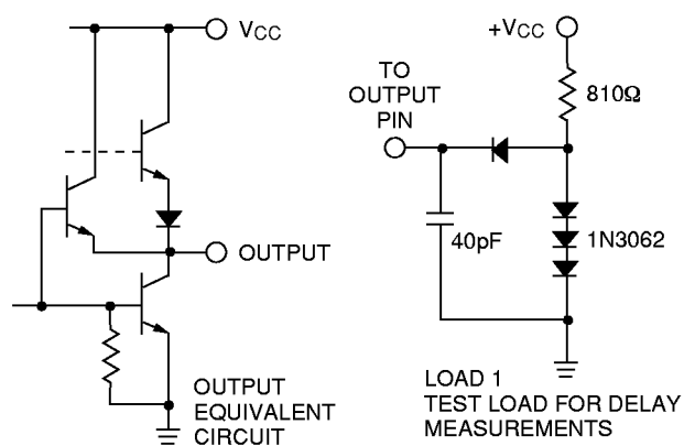
Figure 3. Output Circuits
