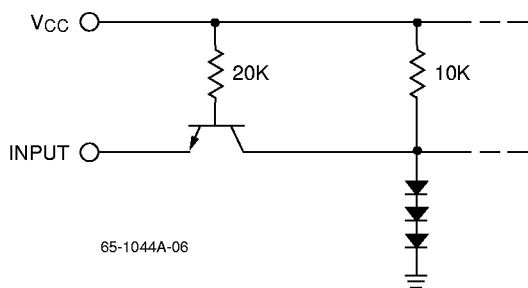
Figure 2. Digital Input Equivalent Circuit
