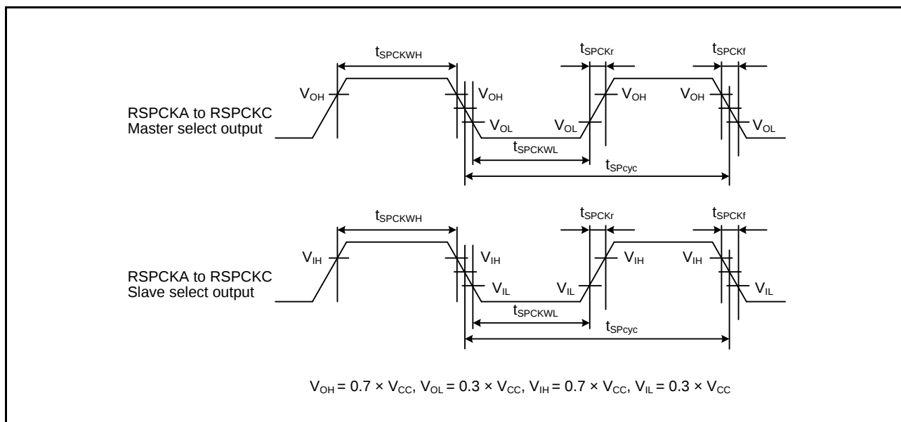
Figure 5.32 RSPCKA to RSPCKC Master select output timing and Simple SPI Clock Timing
