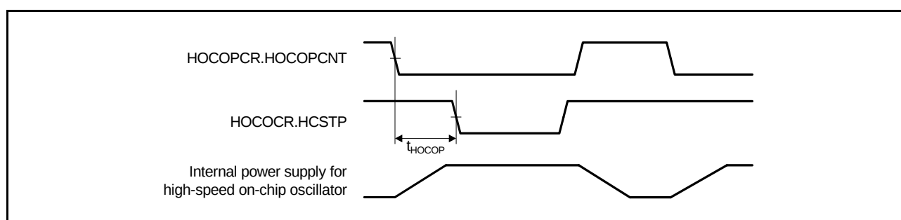
Figure 5.7 High-Speed On-Chip Oscillator Power Supply Control Timing
