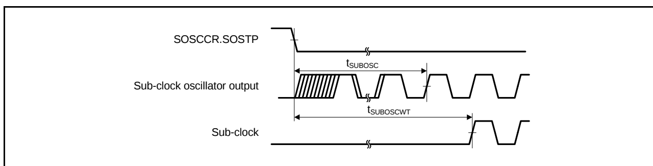
Figure 5.10 Sub-Clock Oscillation Start Timing
