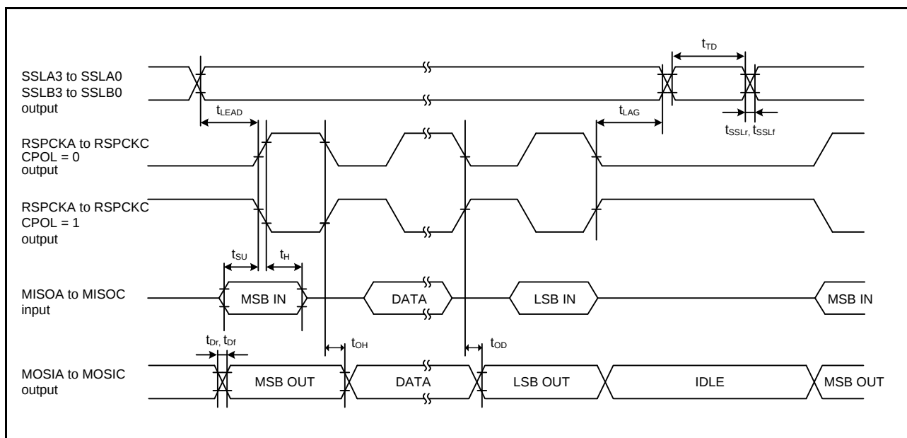
Figure 5.33 RSPCKA to RSPCKC Master, CPHA = 0 and Simple SPI Timing (Master, CPHA = 0)
