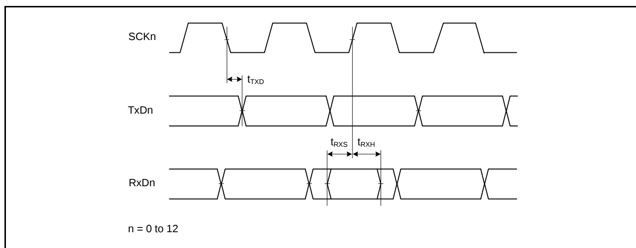
Figure 5.30 SCI Input/Output Timing: Clock Synchronous Mode
