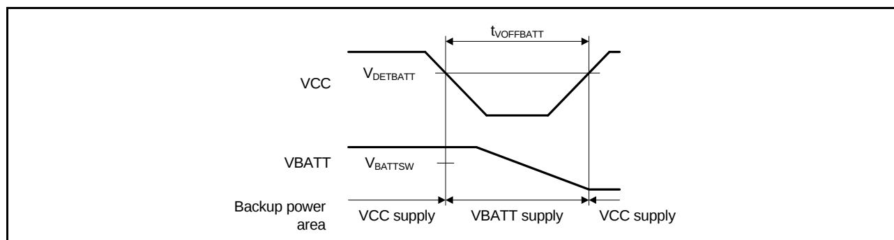
Figure 5.45 Battery Backup Function Characteristics
