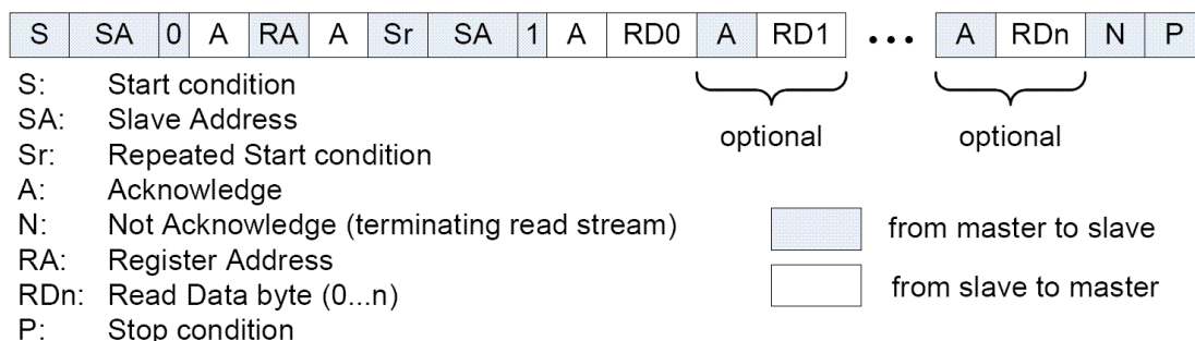
Figure 9 - 2-Wire Serial Interface, Read Operation
