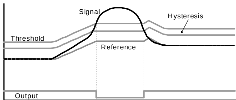
Figure 1.2 Drift Compensation
