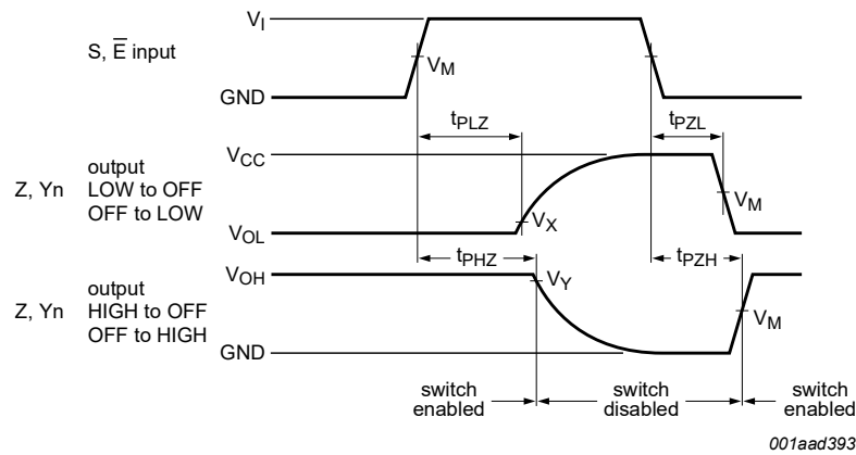
Fig. 14. Enable and disable times
