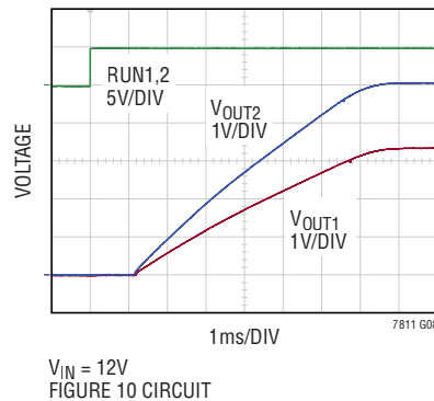
Soft Start-Up
