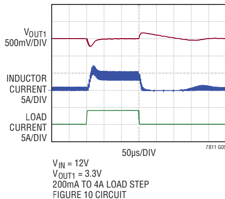
Load Step (Buck) Pulse-Skipping Mode
