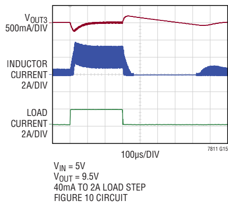
Load Step (Boost) Forced Continuous or Pulse-Skipping Mode
