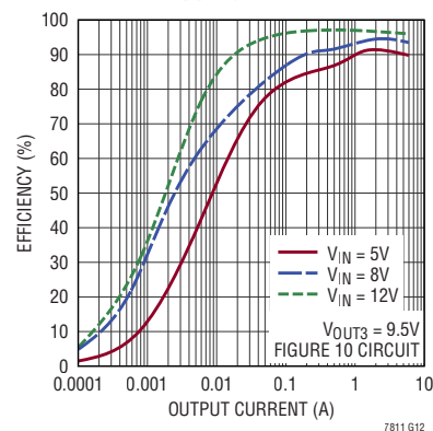
Efficiency vs Output Current (Boost) Pulse-Skipping or Forced Continuous
