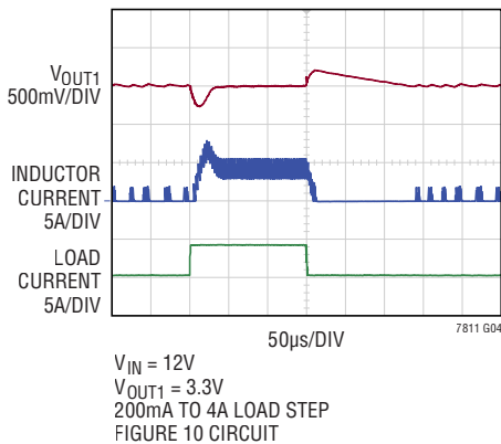
Load Step (Buck) Burst Mode Operation
