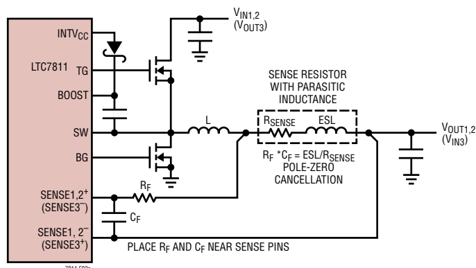
(a) Using a Resistor to Sense Current
