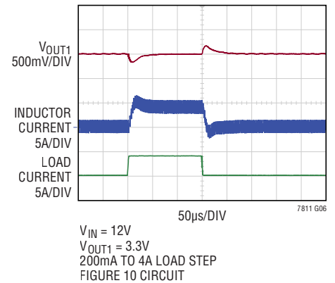
Load Step (Buck) Forced Continuous Mode
