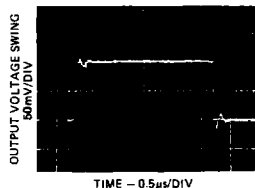
LF155 Small Signal Pulse Response, A_V = +1
