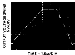
LF155 Large Signal Pulse Response, A_V = +1
