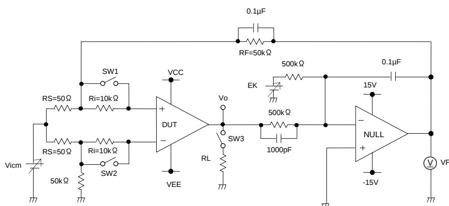
Figure 26. Test circuit1 (one channel only)
