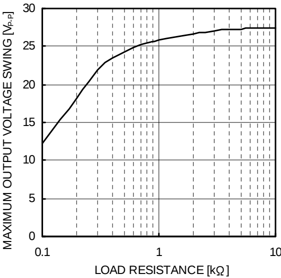
Figure 5. Maximum Output Voltage Swing - Load Resistance (VCC/VEE=+15V/-15V, Ta=25°C)
