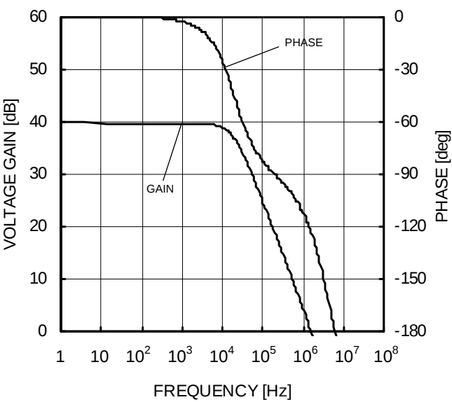
Figure 23. Voltage Gain, Phase - Frequency (VCC/VEE=+15V/-15V, Av=40dB, RL=2kΩ, Ta=25°C)
