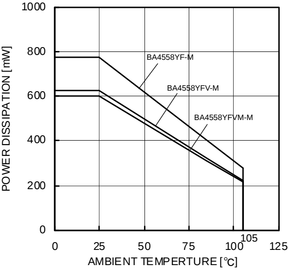
Figure 2. Derating Curve
