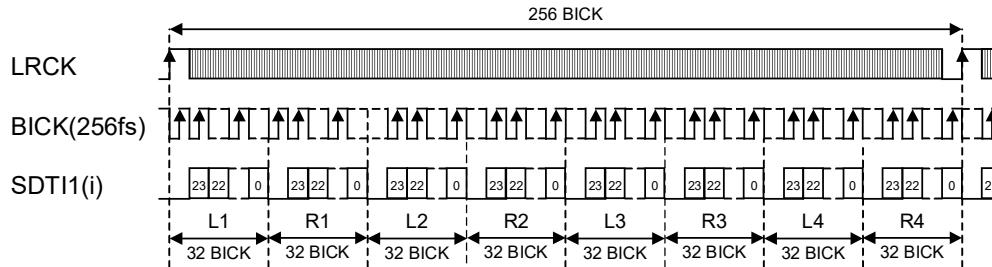
Figure 7. Mode 7 Timing
