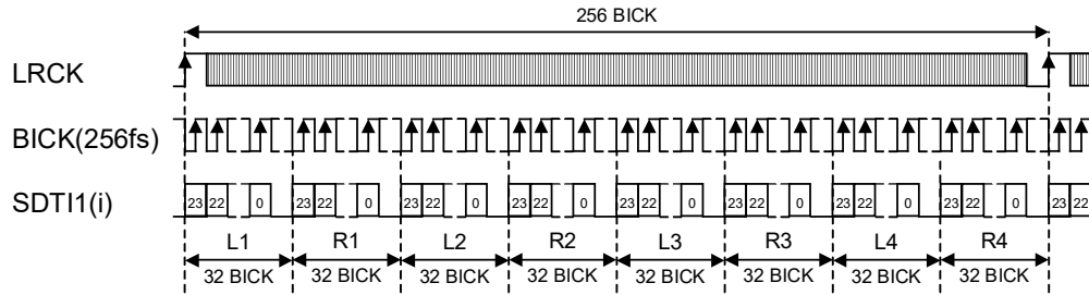
Figure 5. Mode 5 Timing
