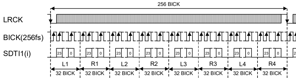
Figure 6. Mode 6 Timing
