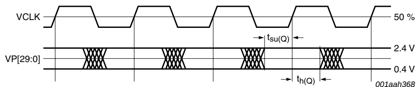
Fig 5. Output timing diagram pin VCLK on pins VP[29:0]
