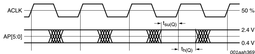
Fig 6. Output timing diagram pin ACLK on pins AP[5:0]
