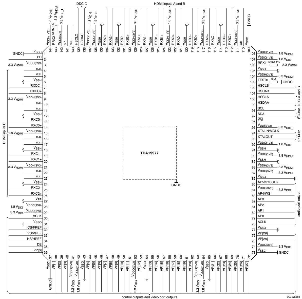
Fig 7. Application diagram of TDA19977A; TDA19977B
