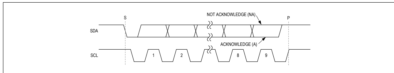
Figure 3. Acknowledge Condition
