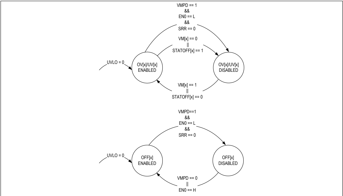
Figure 6. State Diagram
