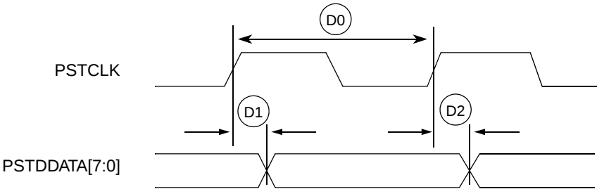
Figure 42. Real-Time Trace AC Timing
