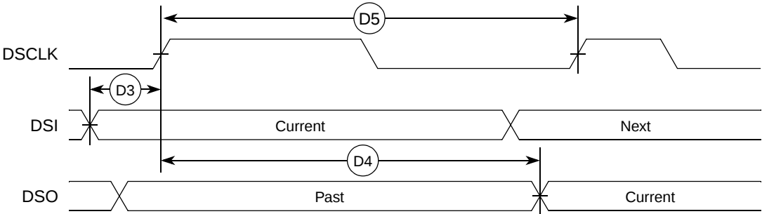
Figure 43. BDM Serial Port AC Timing
