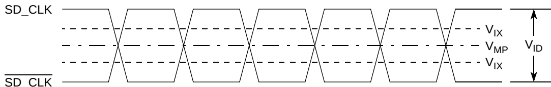
Figure 15. SD_CLK and SD_CLK Crossover Timing
