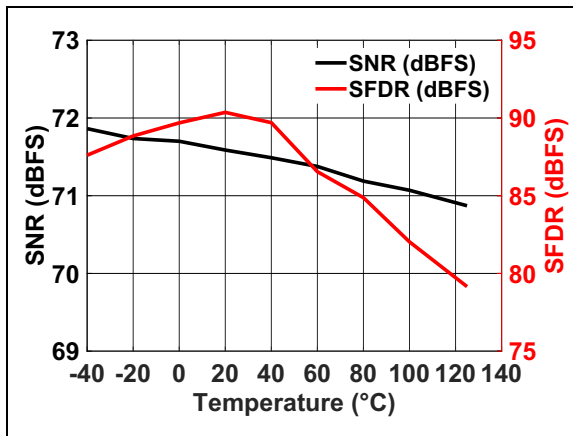
FIGURE 3-36: SNR/SFDR vs. Temperature: f_s = 200 Mps, f_{IN} = 20 MHz, V_{SENSE} = AV_{DD12} , A_{IN} = -1 dBFS.
