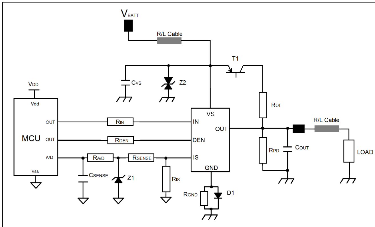
Figure 37. Application Diagram
