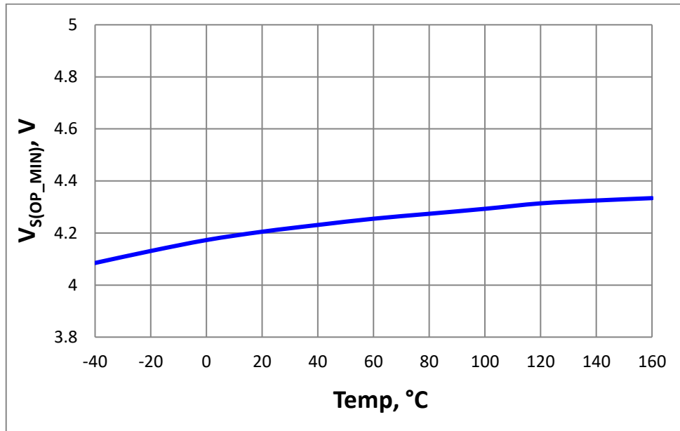
Figure 16. Minimum Functional Supply Voltage V_{S(OP\_MIN)} = f(T_J)
