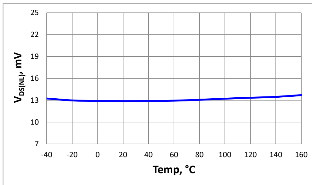
Figure 20. Output Voltage Drop Limitation at Low Load Current V_{DS(NL)} = f(T_J)
