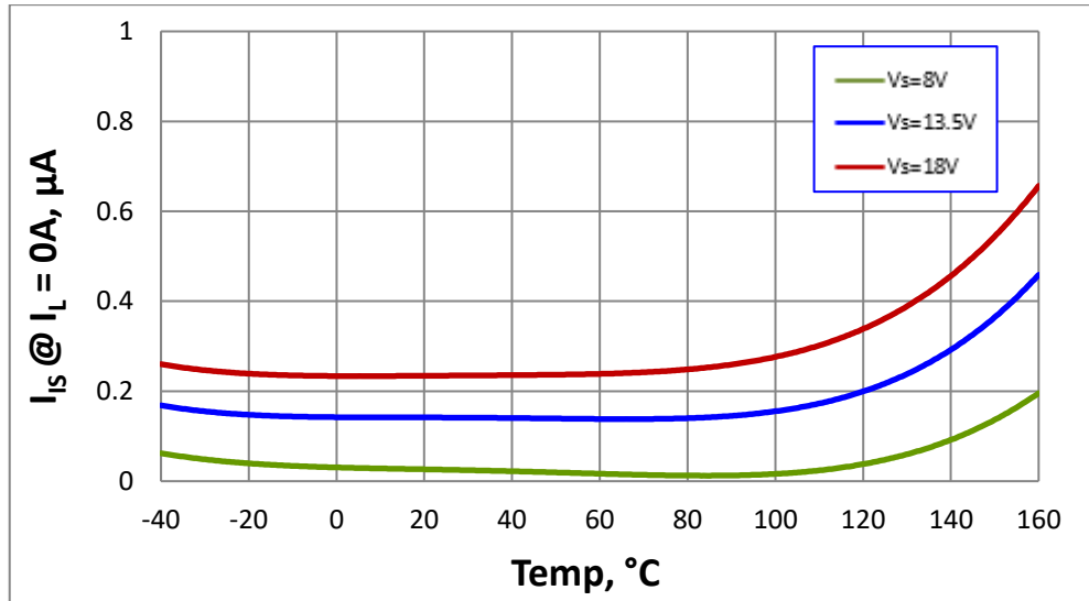
Figure 29. Current Sense at No Load I_s = f(T_j; V_s)
