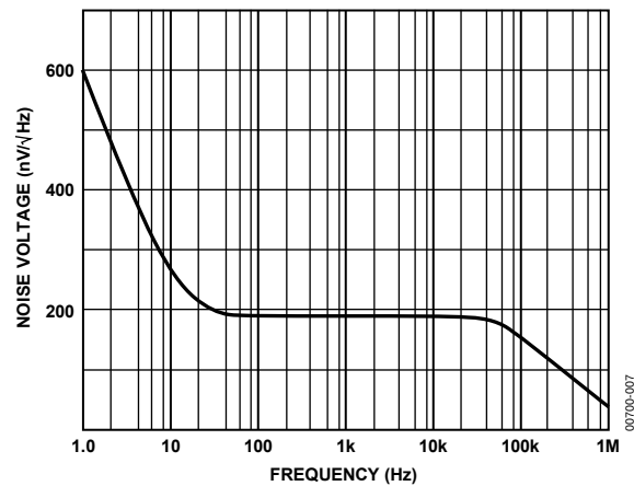
Figure 7. Noise Spectral Density
