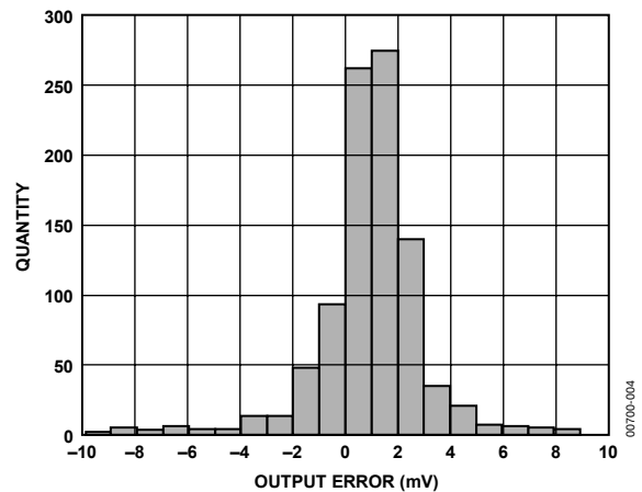
Figure 4. Reverse Voltage Error Distribution
