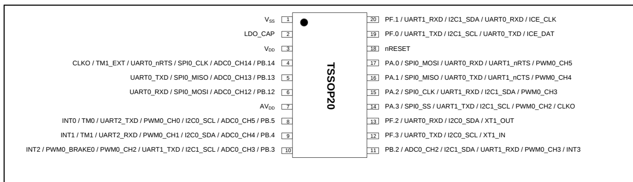
Figure 4.1-7 M031FB0AE Multi-function Pin Diagram
