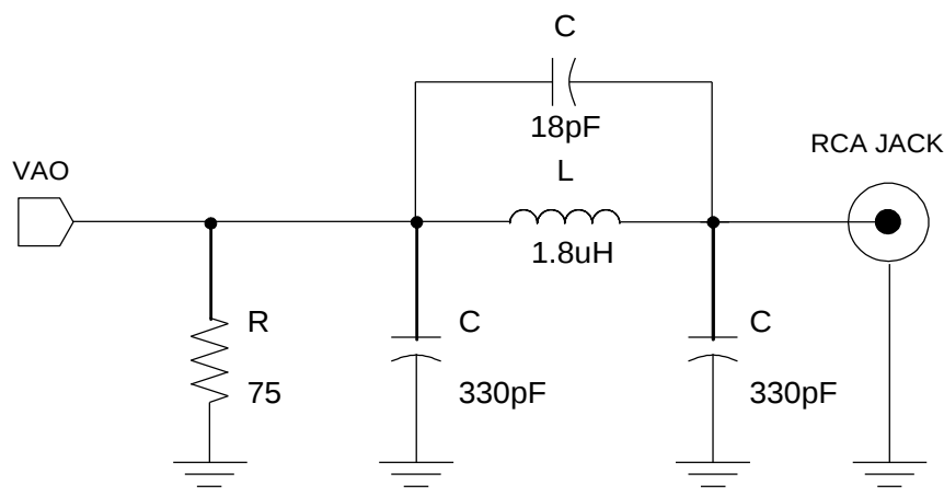
FIGURE 23. EXAMPLE OF RECONSTRUCTION FILTER
