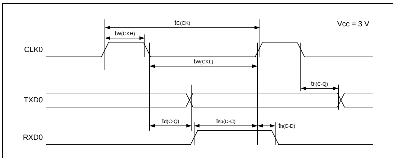
Figure 4.10 Serial Interface Timing When V_{CC} = 3\text{ V}
