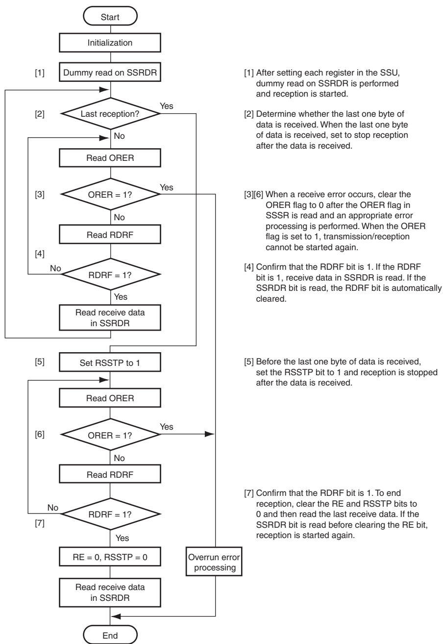
Figure 25.8 Sample Serial Reception Flowchart (MSS = 1)
