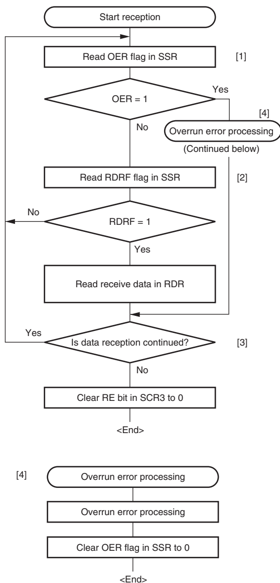
Figure 21.15 Sample Flowchart for Data Reception (Clocked Synchronous Mode)
