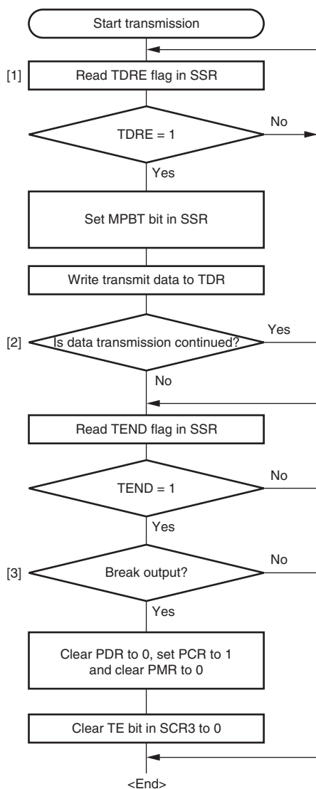
Figure 21.18 Sample Flowchart for Multiprocessor Data Transmission
