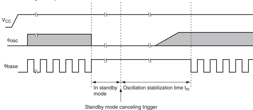
Figure 31.3 Oscillation Stabilization Time Timing
