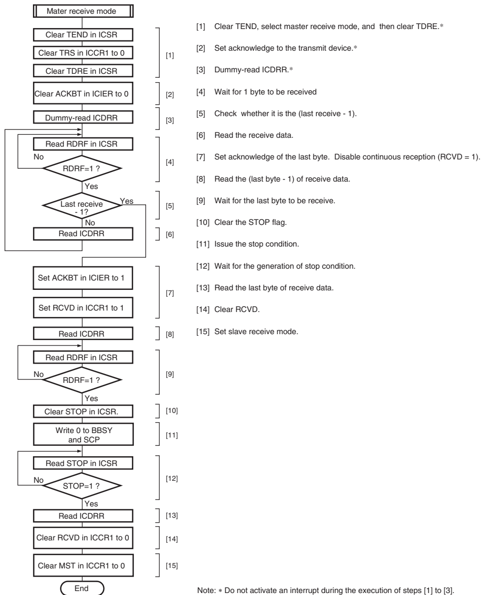
Figure 24.18 Sample Flowchart for Master Receive Mode
