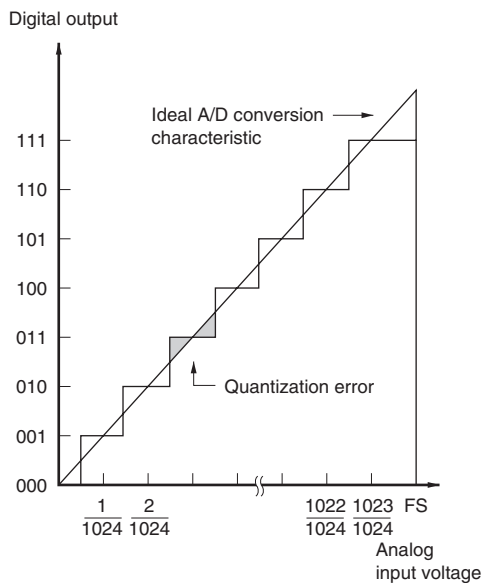
Figure 27.9 A/D Conversion Accuracy Definitions
