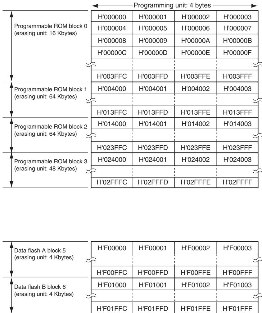
Figure 7.1 Block Configuration of Flash Memory (4)
