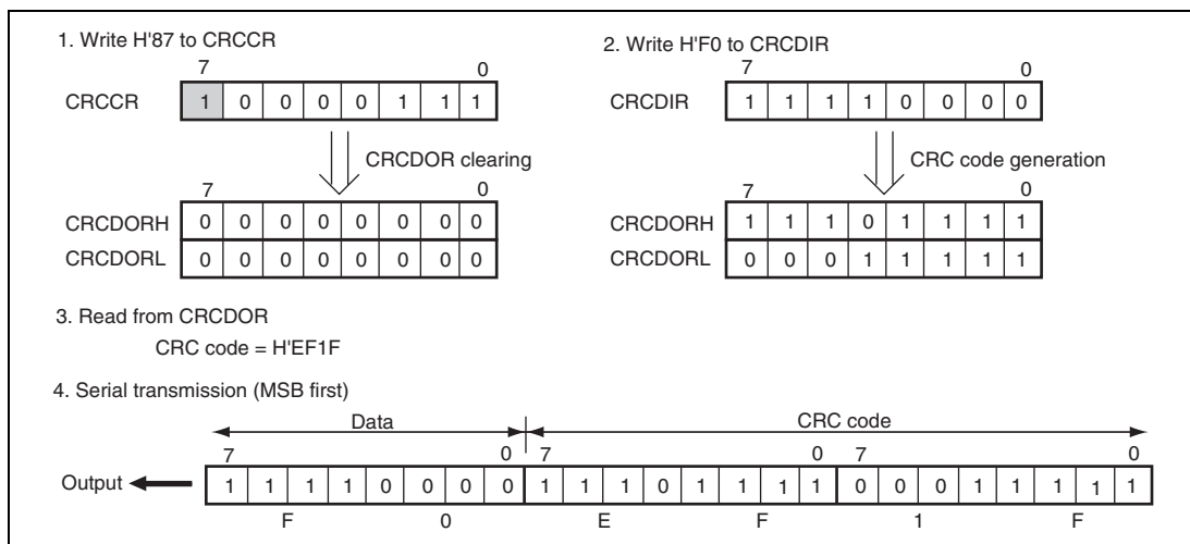
Figure 23.3 MSB-First Data Transmission
