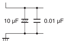
Figure 27.12 Example of Analog Input Protection Circuit
