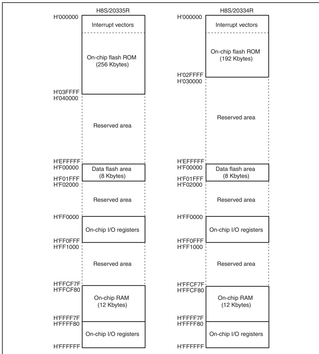
Figure 2.3 Memory Map (8) (H8S/2035R Group)
