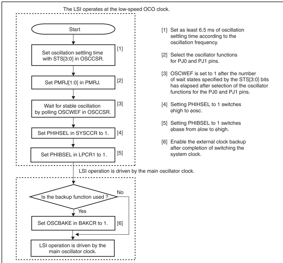
Figure 5.6 Flowchart of Clock Switching from \phi_{loco} to \phi_{osc} (2)
