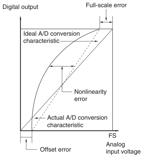
Figure 27.10 A/D Conversion Accuracy Definitions
