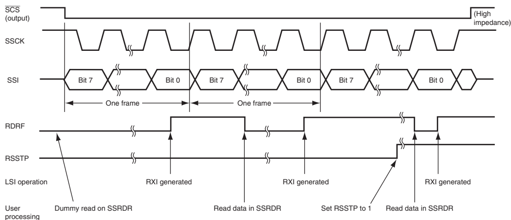
Figure 25.12 Example of Operation in Data Reception (MSS = 1)
