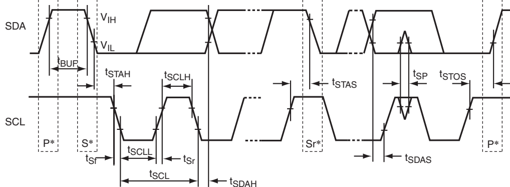
Figure 31.4 Input Timing
