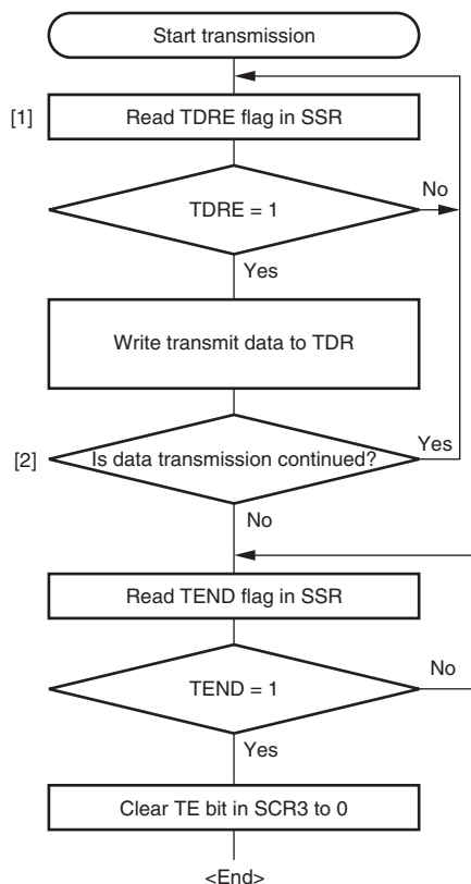
Figure 21.13 Sample Flowchart for Data Transmission (Clocked Synchronous Mode)
