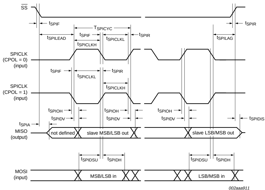
Fig 39. SPI slave timing (CPHA = 1)
