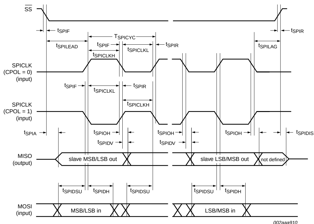
Fig 38. SPI slave timing (CPHA = 0)
