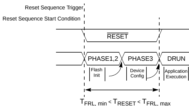
Figure 24. Functional reset sequence long
