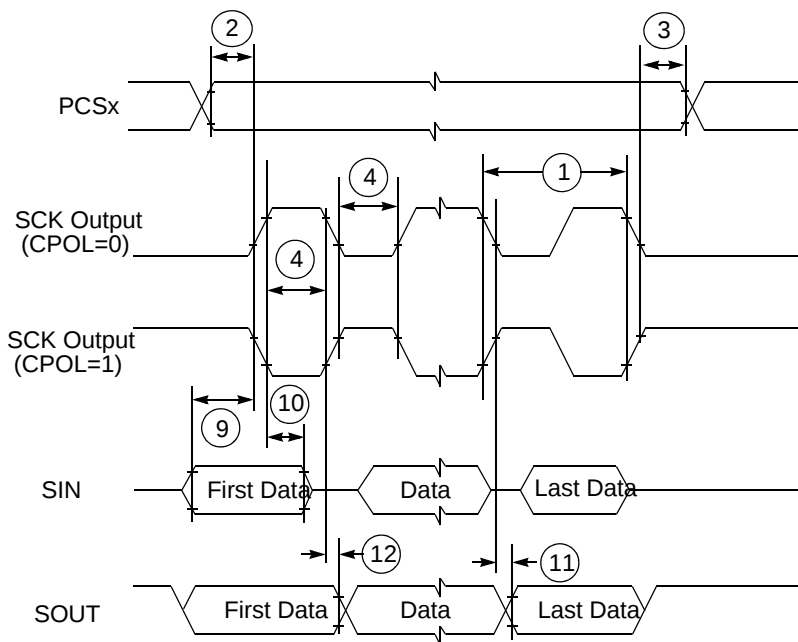
Figure 40. DSPI classic SPI timing—master, CPHA = 0
