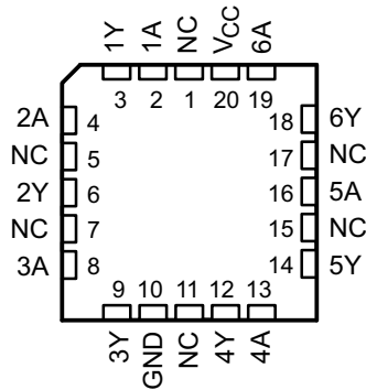
Figure 5-3. SN54AHCT14 FK Package, 20-Pin LCCC (Top View)
