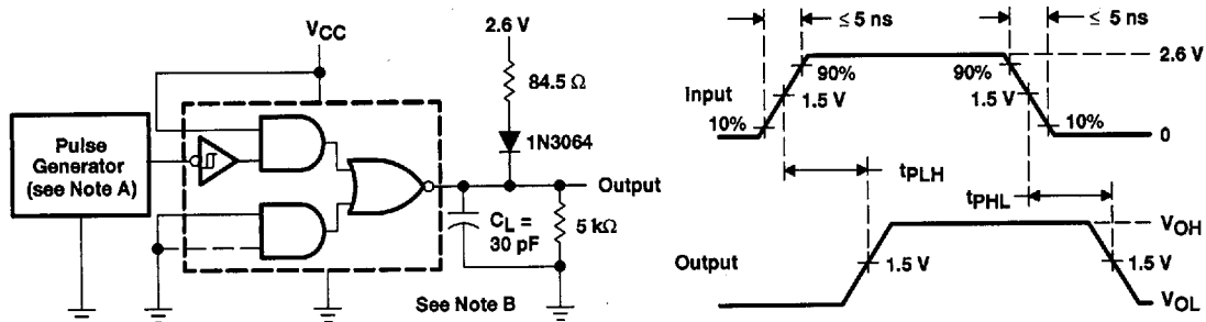
VOLTAGE WAVEFORMS
