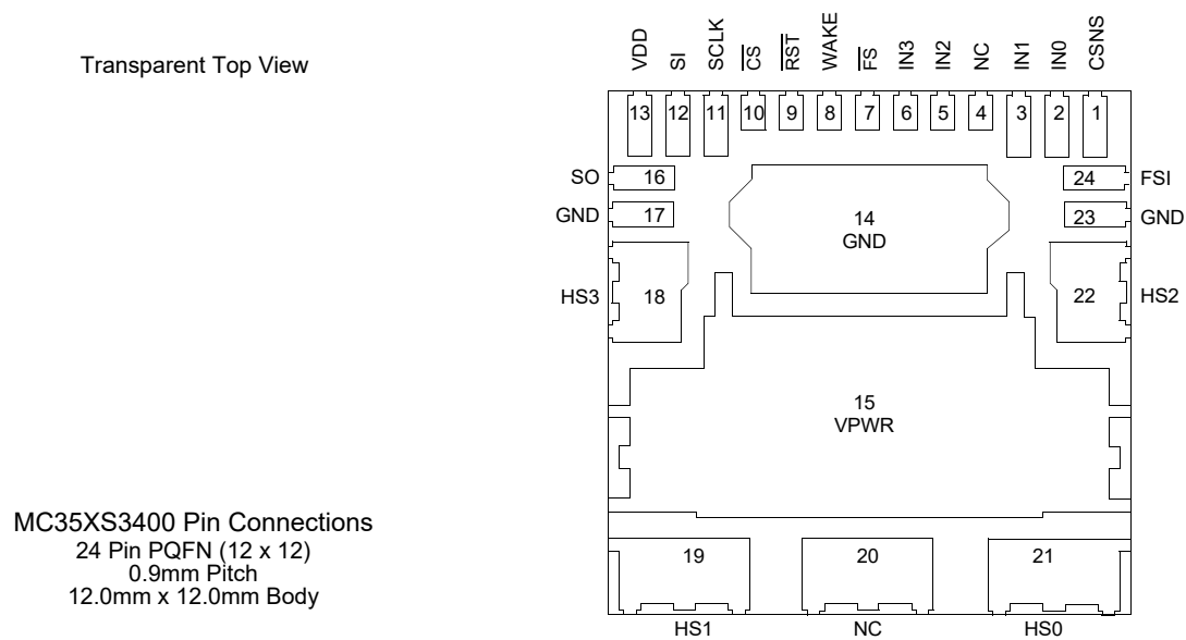
Figure 22. Pin connections
