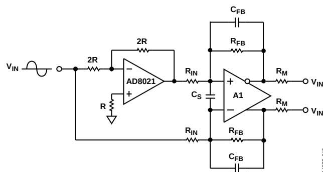
Figure 27. Single-Ended-to-Differential Conversion
