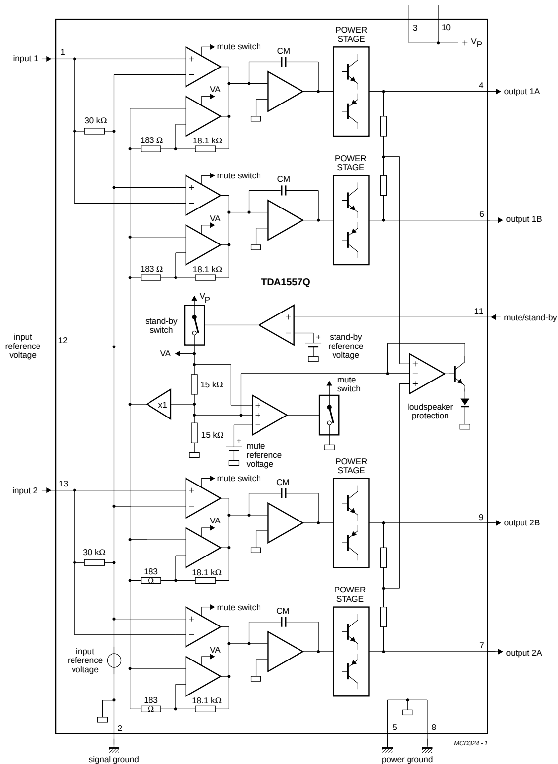
Fig.1 Block diagram.
