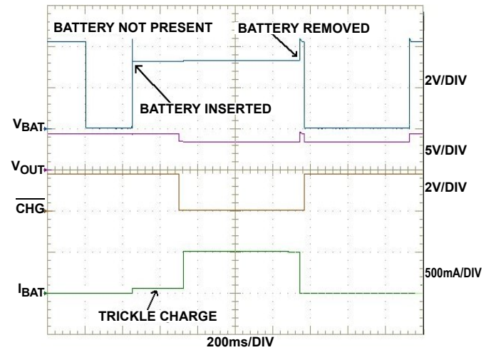
FIGURE 5. BATTERY DETECTION - BATTERY INSERTED/REMOVED
