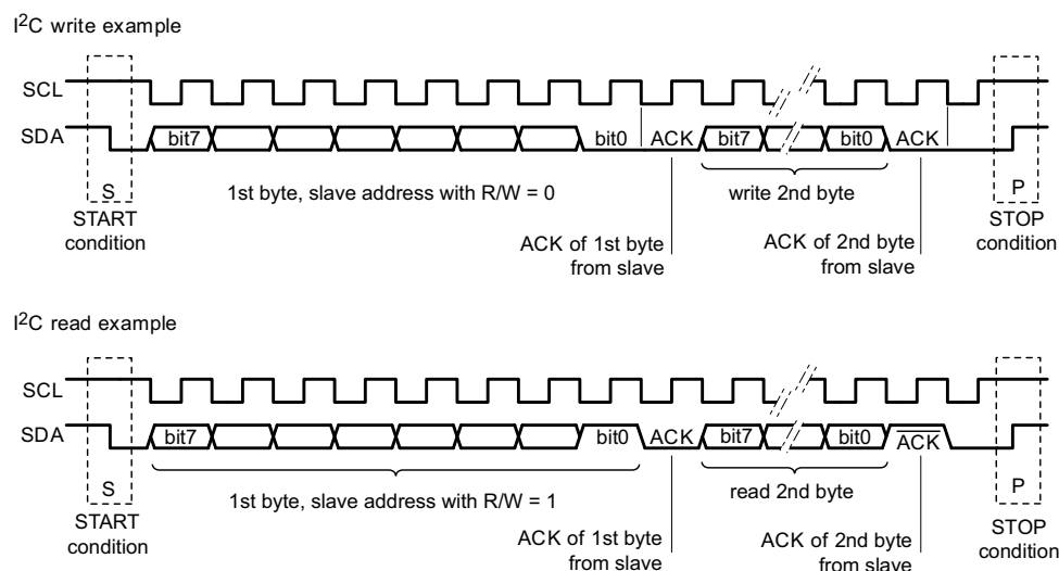
Fig 34. I 2 C read and write signaling
