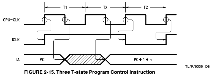
FIGURE 2-15. Three T-state Program Control Instruction
