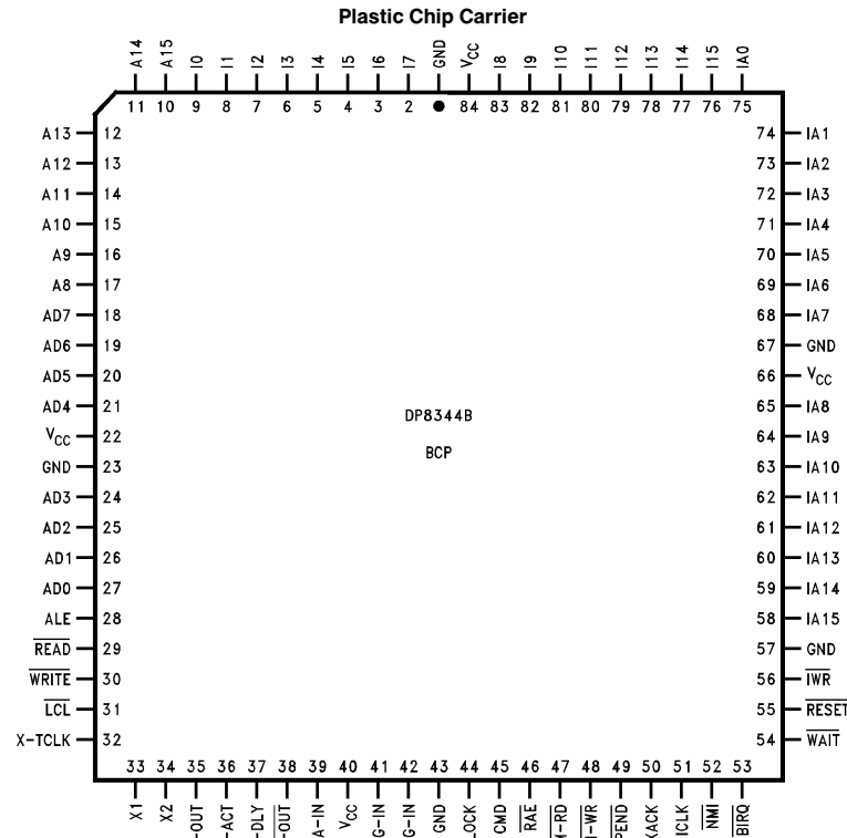
FIGURE 5-1. Top View
