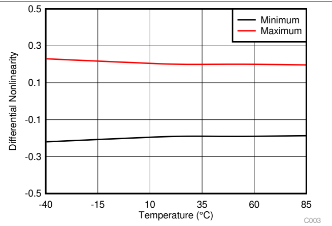
Figure 3. Typical DNL
