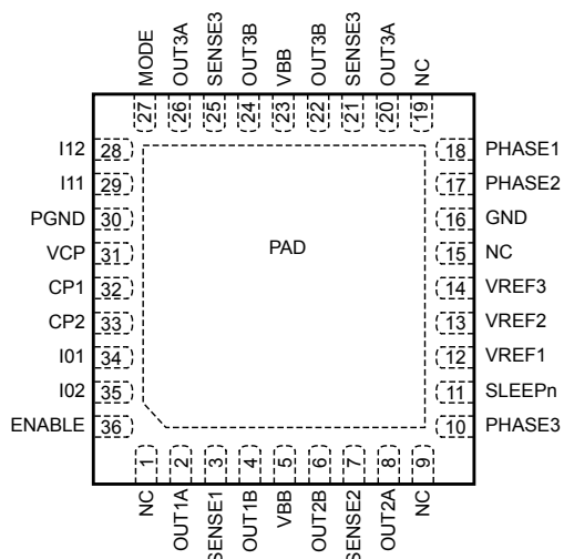
Pinout Diagram
