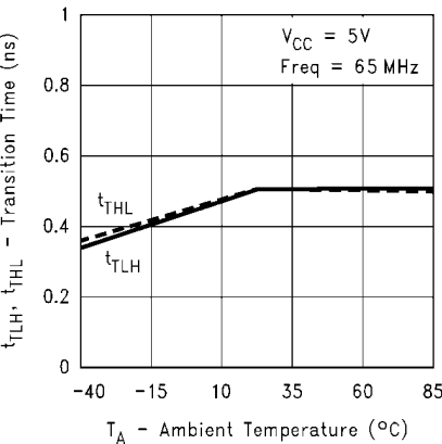
Transition Time vs Ambient Temperature
