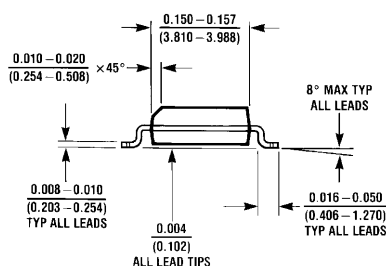
16-Lead (0.150" Wide) Molded Small Outline Package, JEDEC Order Number DS90C032TM NS Package Number M16A
