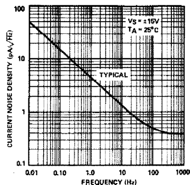
INPUT SPOT NOISE CURRENT vs FREQUENCY
