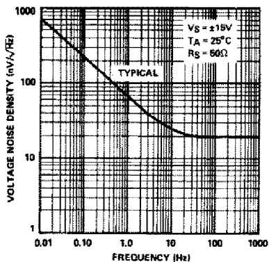
INPUT SPOT NOISE VOLTAGE vs FREQUENCY
