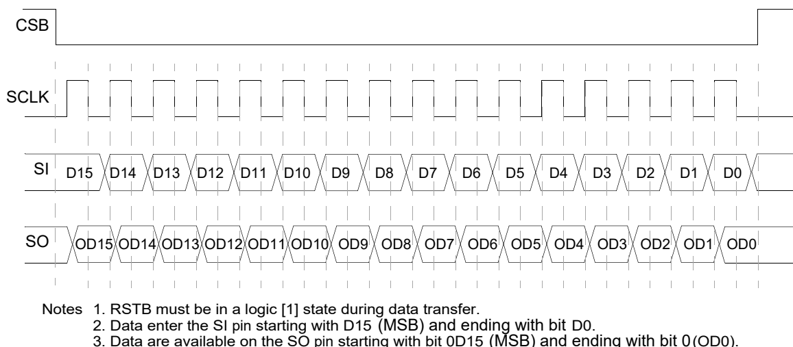
Figure 22. 16-bit SPI interface timing diagram
