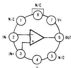
HA2-5151 (TO-99 METAL CAN)
