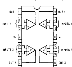
HA1-5154 (CERAMIC DIP) HA3-5154 (PLASTIC DIP)
