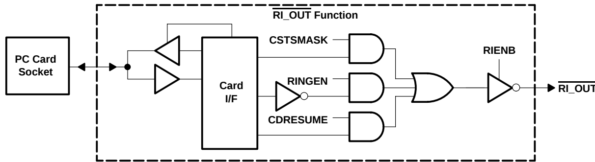
Figure 3-19. \overline{\text{RI\_OUT}} Functional Diagram
