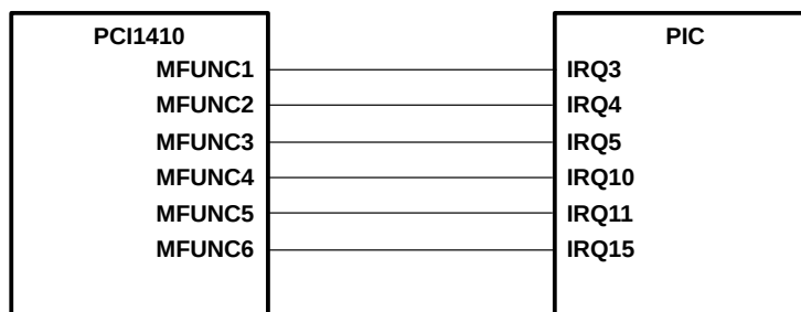
Figure 3–16. IRQ Implementation
