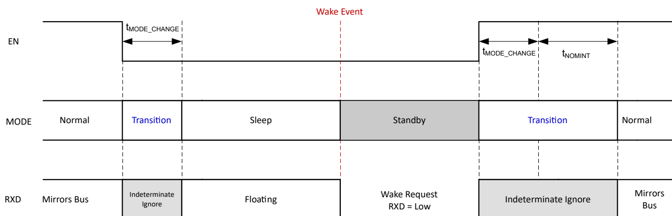
Figure 8-15. Mode Transitions
