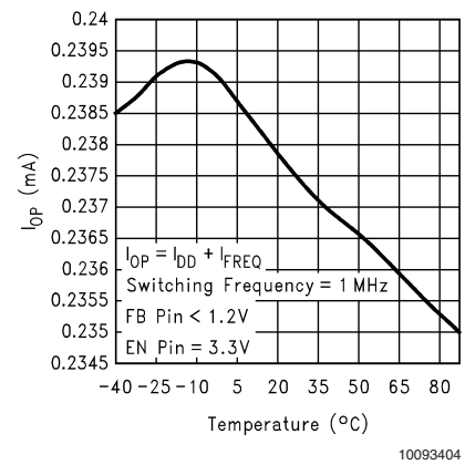
I_{OP} vs Temperature
